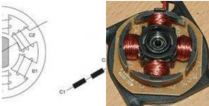
Fig. 5 The connection of rotor and stator's winding for BLDC motor.
